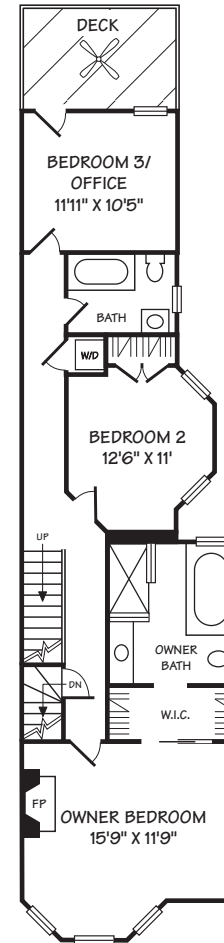
SECOND LEVEL 9' CEILING
