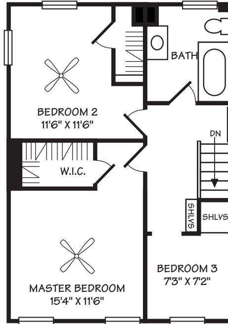
SECOND LEVEL 8' CEILING
